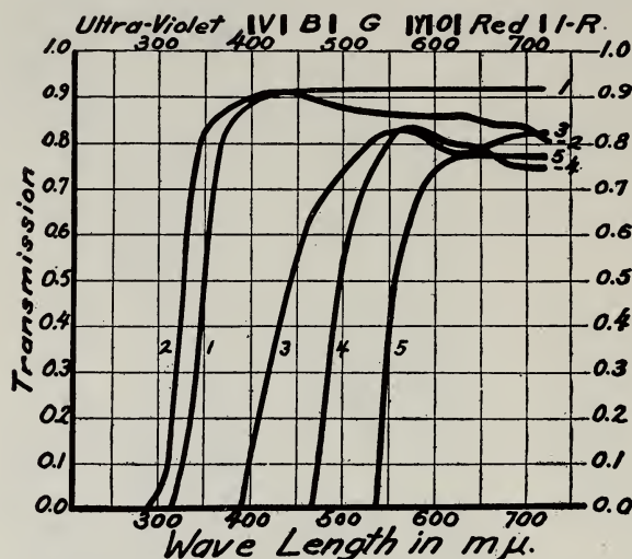
FIGURE 128. Transmission curves of glasses in the visible and ultraviolet. Figures on curves represent house numbers: 1, is ordinary greenhouse glass (house 1); 2, is Corning glass G86B (house 2); 3, is Corning's Noviol O (house 3); 4, is Corning's Noviol C (house 4); 5, is Corning glass G34 (house 5).
