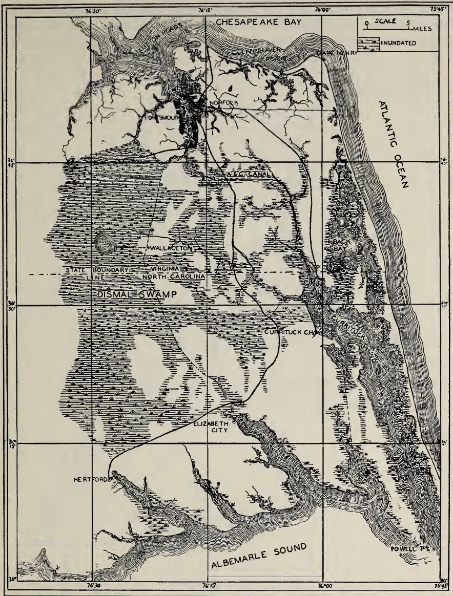
FIGURE 6. The Back Bay, Virginia, and Currituck Sound, North Carolina, region, showing the relation of these waters to the Albemarle and Chesapeake Canal, Norfolk Harbor, and Hampton Roads.
