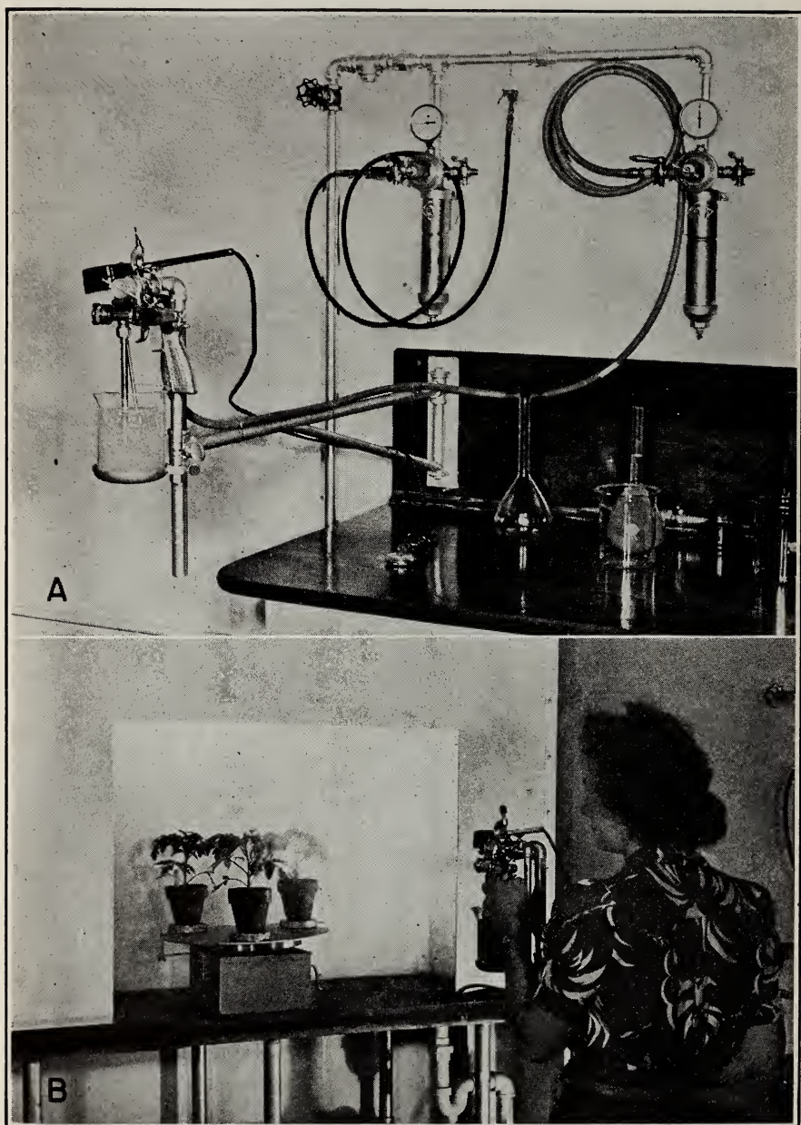
FIGURE 148. A, Spraying systems. Upper left : low pressure for inoculation; upper right : high pressure for applying fungicide. Note swinging arm mounting spray gun, height adjustment, attached stirrer, and rimmed plate holding beaker containing fungicide. B, Spraying tomato plants on compound turntable in hood, with fungicide at 40 lbs pressure.
