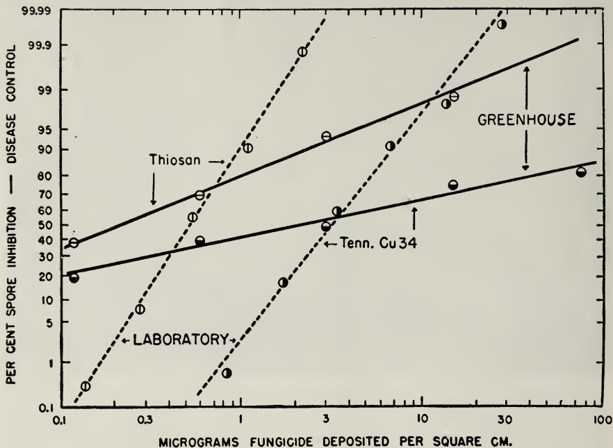
FIGURE 150. Absolute comparison of laboratory and greenhouse dosage-response curves; identical fungus and fungicides. Tennessee Copper "34" and Thiosan against early blight ( Alternaria solani Maine strain). Spore concentration constant, 70 per sq cm.
