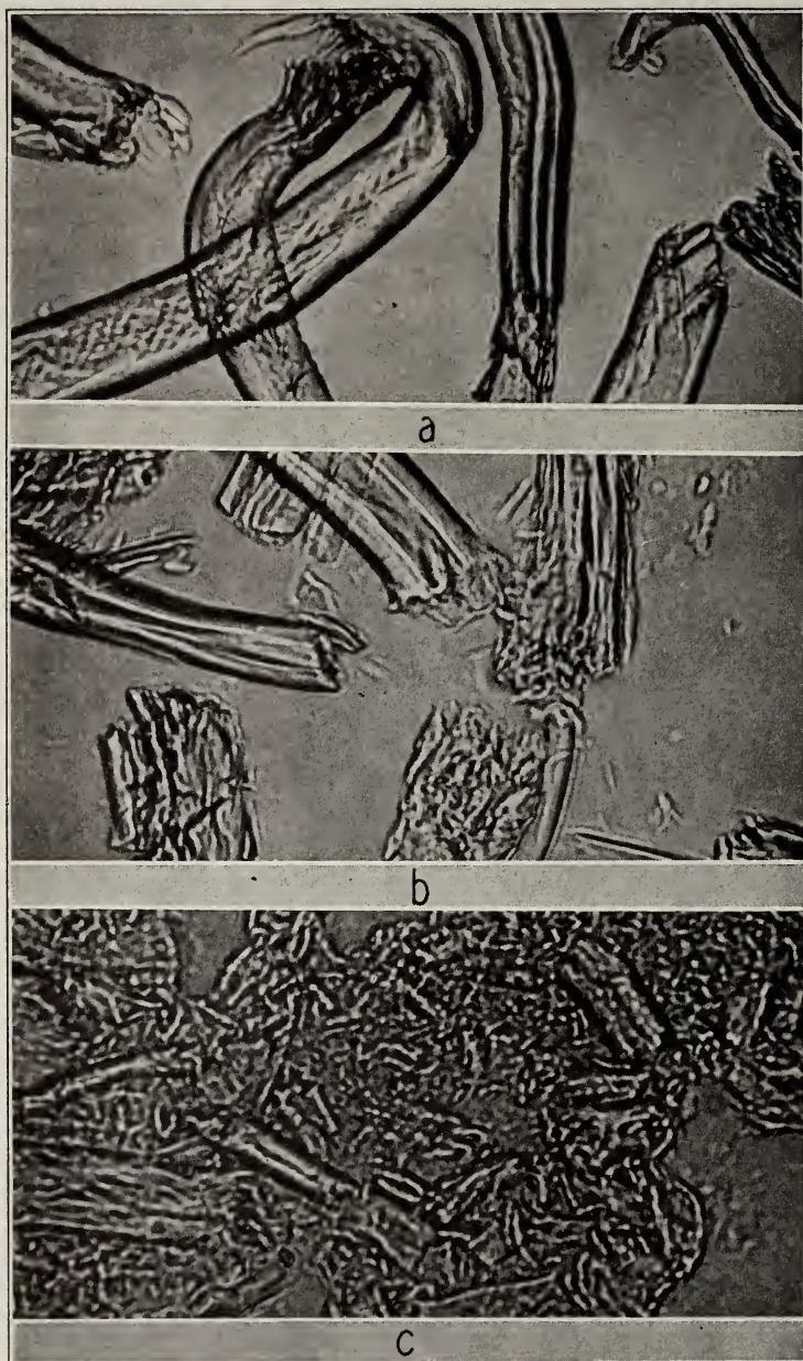
FIGURE 101. a , Portions of fibers from the residues after treatment for 2\frac{1}{2} hours with HCl. The fibril and particle structure of the membranes are shown as well as the cross-sectional rupturing of the fiber (350 \times ). b , More advanced degree of fiber dissociation after 18 hours' treatment with HCl (350 \times ). c , Extreme degree of fiber dissociation after 5 days' treatment with HCl (350 \times ).
